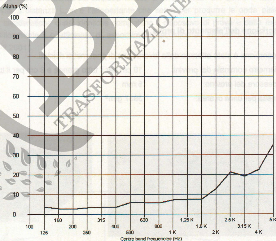
Alpha (1/3 octave)
